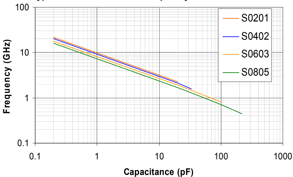
Typical Series Resonant Frequency of aec GP Series NPO MLCC
