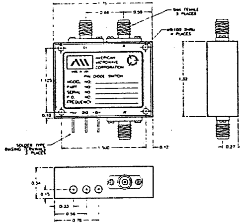
FIGURE 3. DC Power Supply : \pm 5\text{vdc} @ \pm 60\text{mA} Max. ● SWN-1TDR-ARG-LVT
