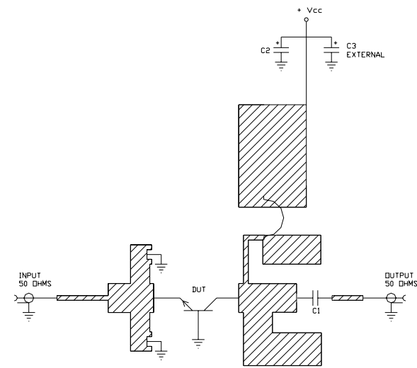
ELECTRICAL SCHEMATIC
