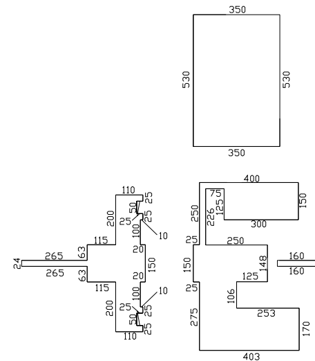
CIRCUIT DIMENSIONS IN MILS (1 MIL = 0.001")
