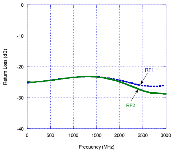
Figure 12. Return Loss – RFC to RF1, RF2
