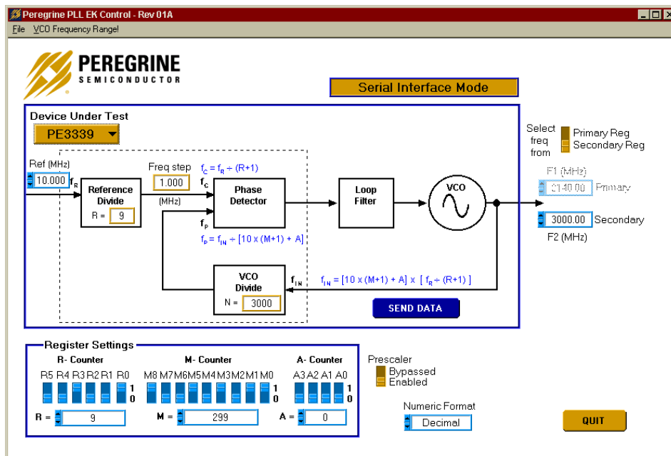
Figure 4. PE3339 Software Control Panel
