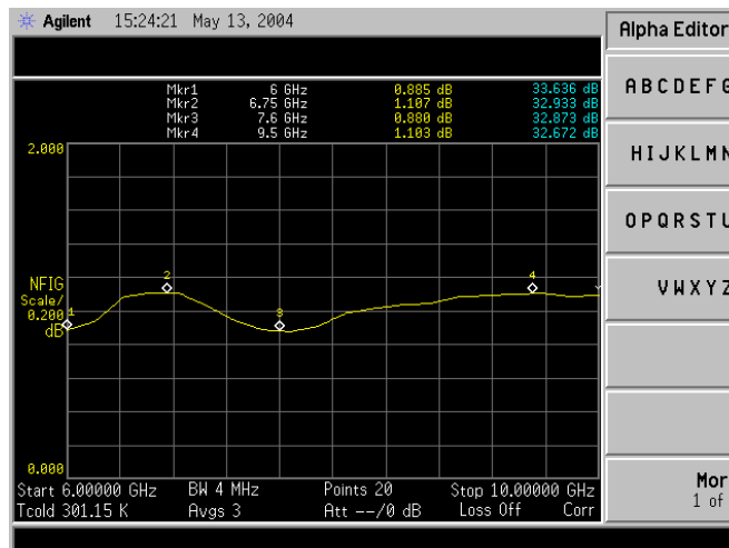
Below: 6-10 GHz Noise Figure Measurement
