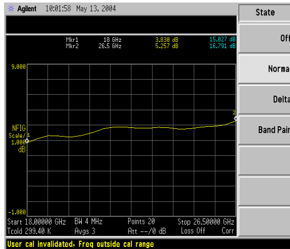
Below: 18-26.5GHz Noise Figure Measurement
