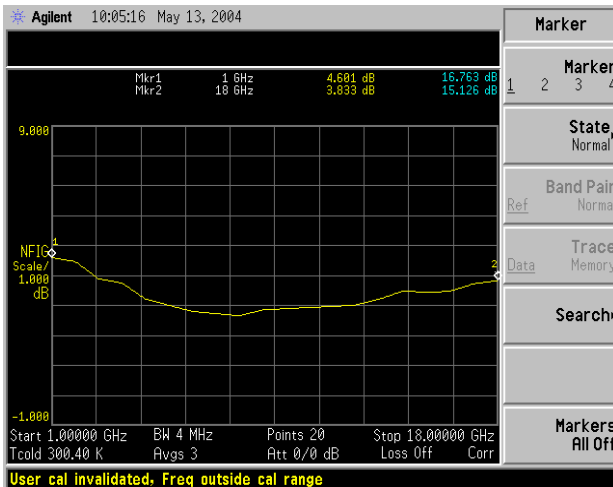
Below: 1-18GHz Noise Figure Measurement
