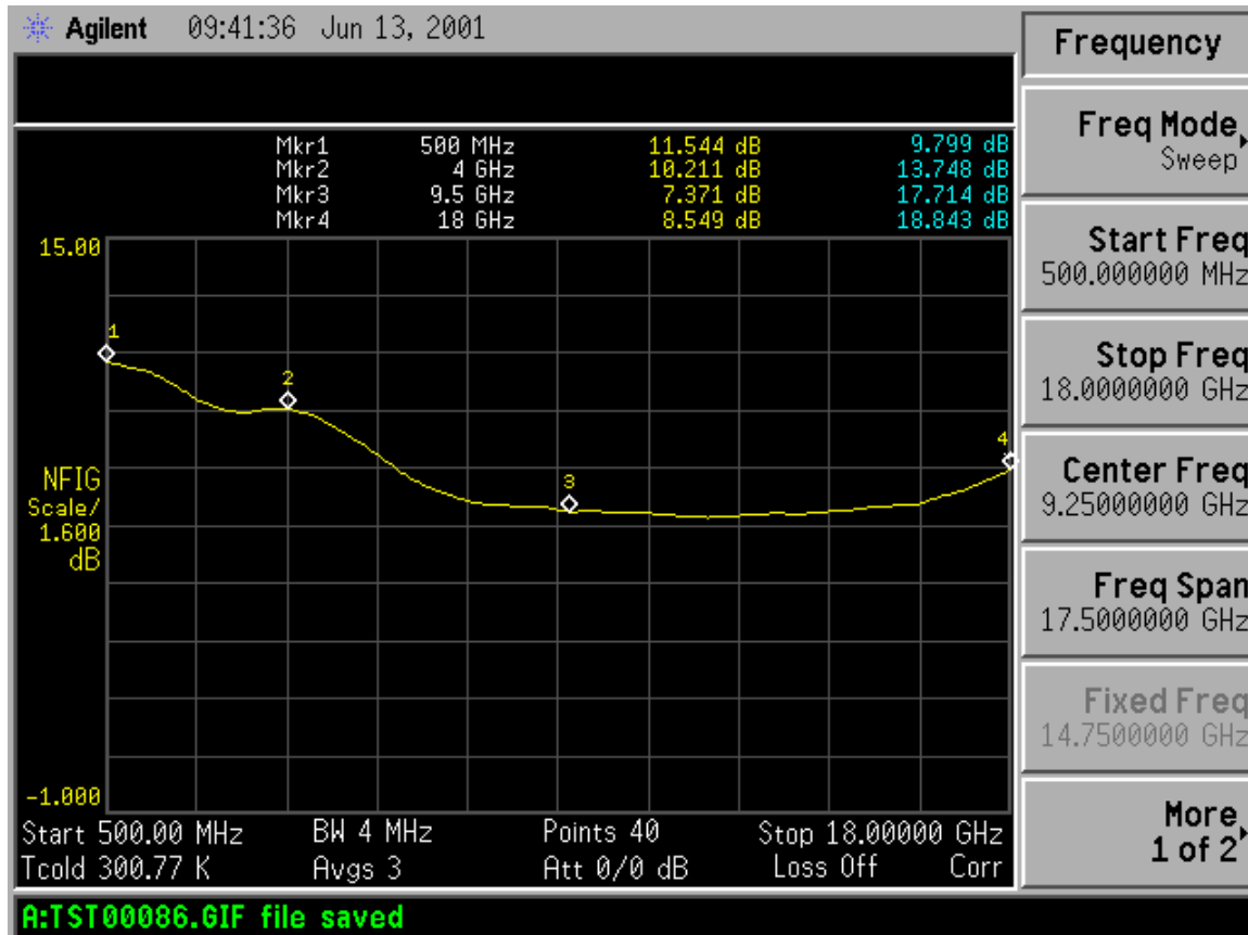
Noise Figure Plot
