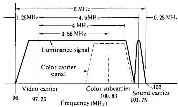
(Fig. 2) Frequency Spectrum In TV Wave
