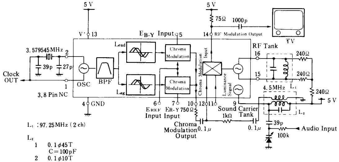
Fig. 4 APPLICATION OF BASE-BAND OUTPUT
