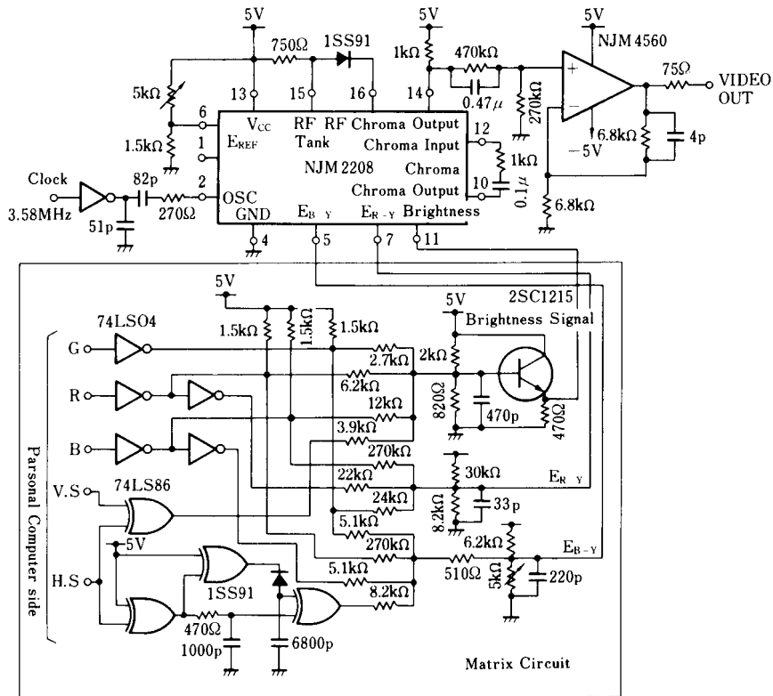
Fig. 4 APPLICATION OF BASE-BAND OUTPUT
