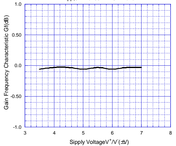
Gain Frequency Characteristic Gf (dB) vs. Supply Voltage
