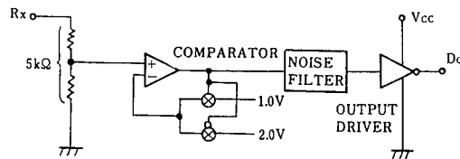
(2) Receiver Section ( 1-circuit )
