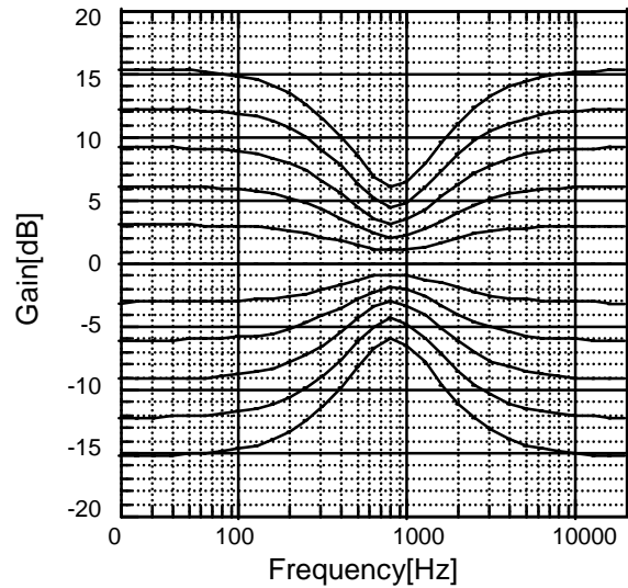
Tone Control
