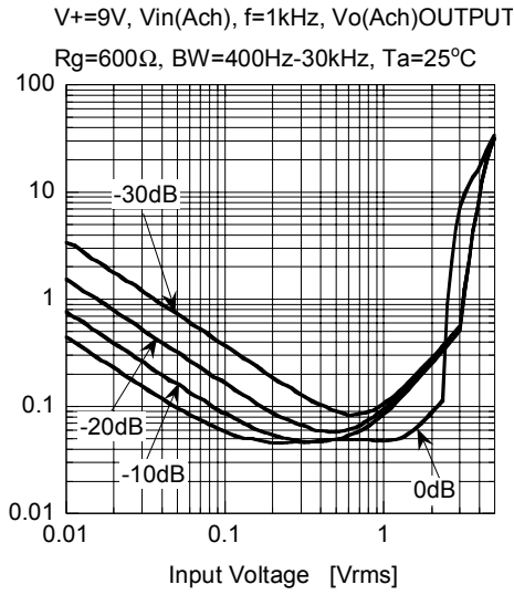
THD+N vs Input Voltage
