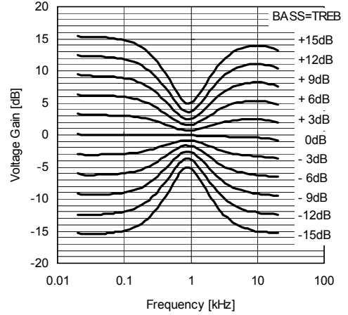
Voltage Gain vs. Frequency (BBE)
