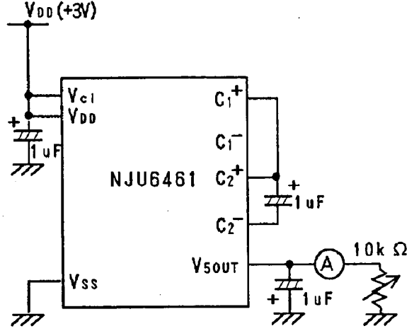
Voltage Tripler/Doubler Operation Clock Frequency = 1.25kHz (fosc=80kHz)
