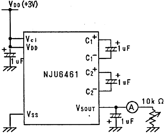
Voltage Tripler/Doubler Operation Clock Frequency = 1.25kHz (fosc=80kHz)
