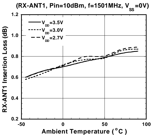
Loss vs. Ambient Temperature
