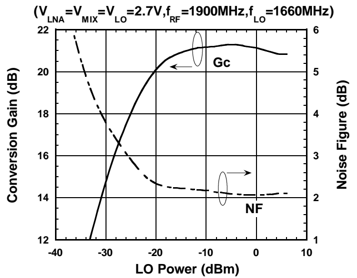
Conversion Gain , Noise Figure vs. LO Power
