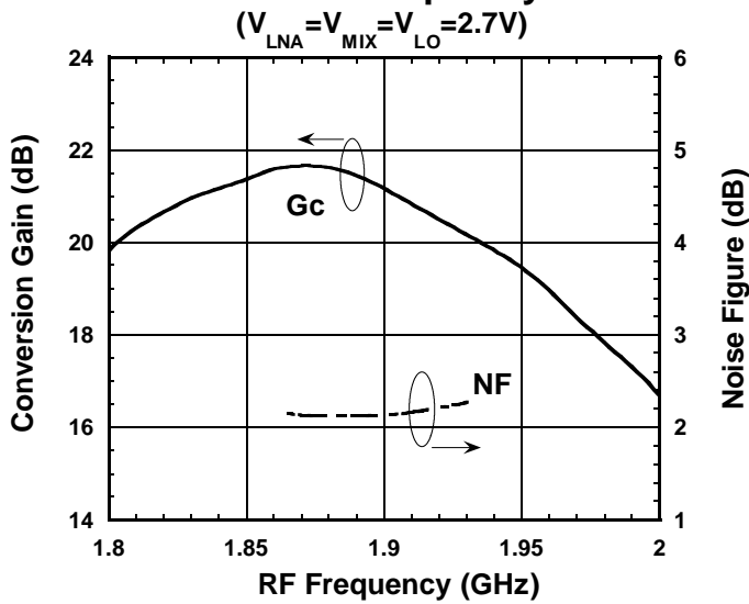
Conversion Gain , Noise Figure vs. RF Frequency
