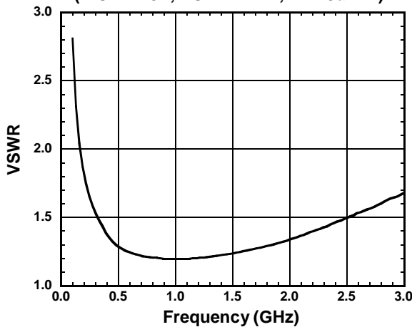
P1 VSWR vs. Frequency
