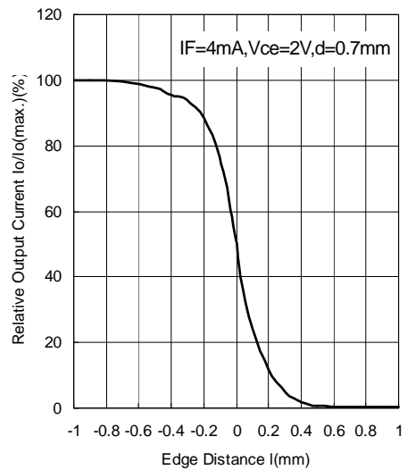
Output Current vs. Edge Distance ( T_a=25^\circ\text{C} )
