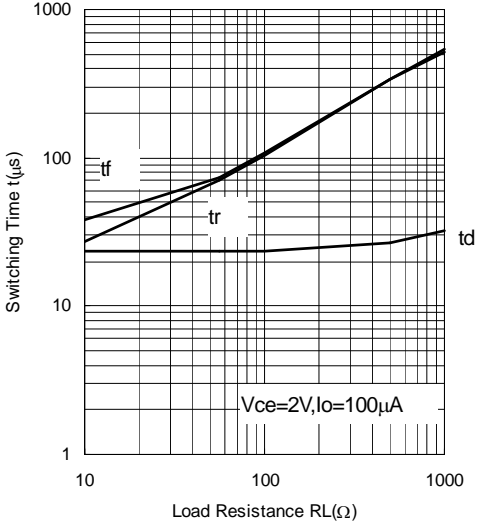
Switching Time vs. Load Resistance (Ta=25°C)
