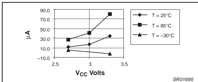
Figure 11. Sleep current
