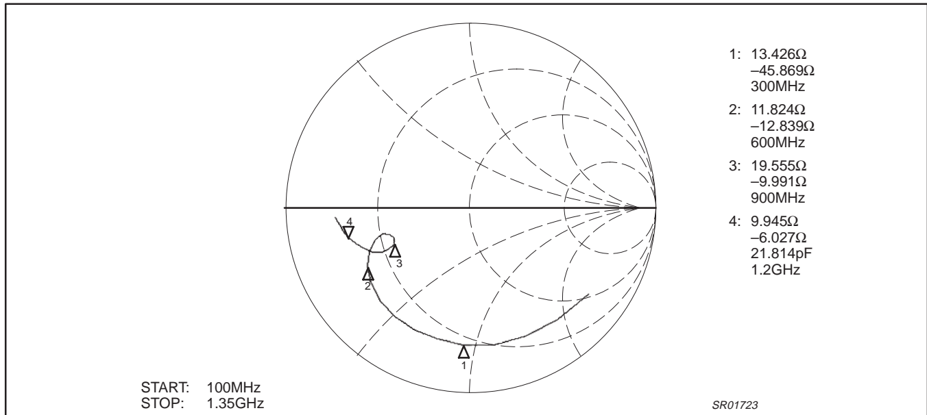
Figure 16. Typical S 11 of LO Input @ V CC = 2.8V
