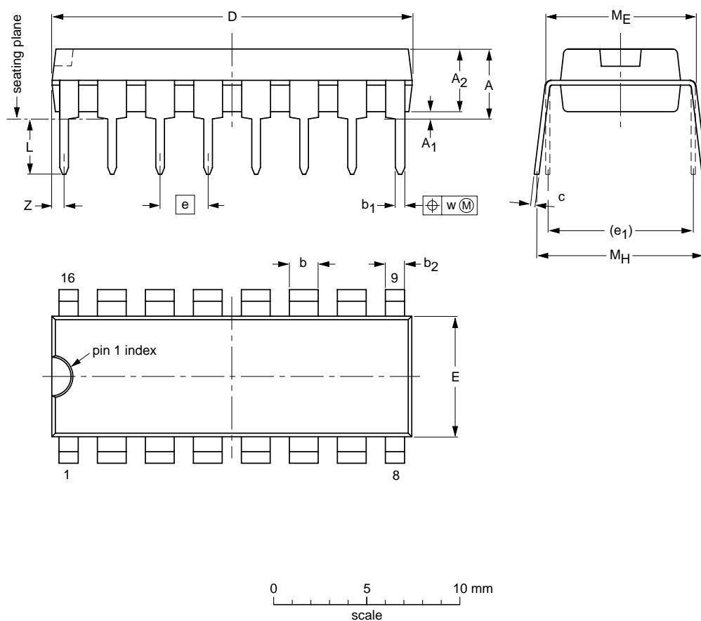
DIMENSIONS (mm dimensions are derived from the original inch dimensions)
