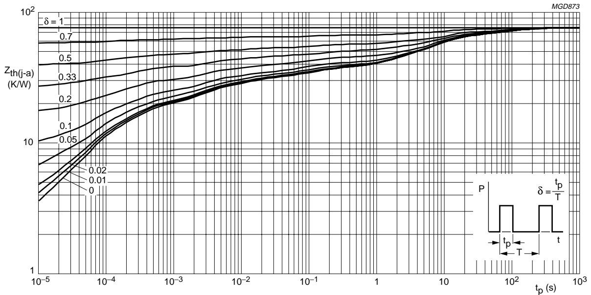
Fig.10 Thermal impedance curves (junction to ambient) for transistors mounted on a printed-circuit board: SOT89.
