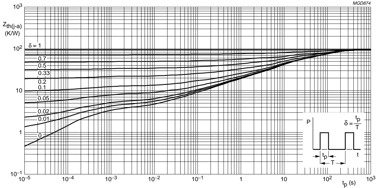
Fig.9 Thermal impedance curves (junction to ambient) for transistors mounted on a printed-circuit board: SOT89.
