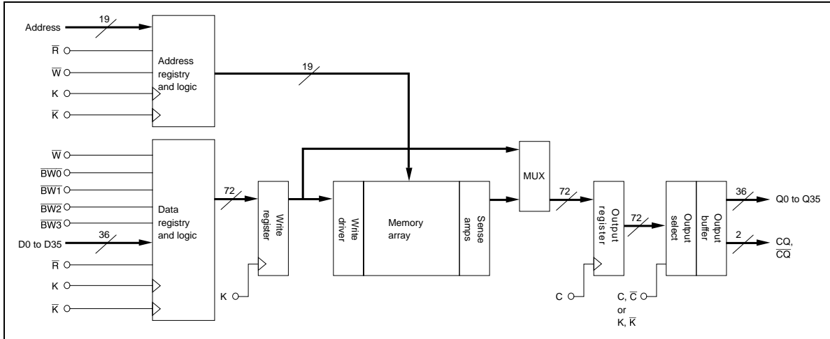
Block Diagram (HM66AQB36102)
