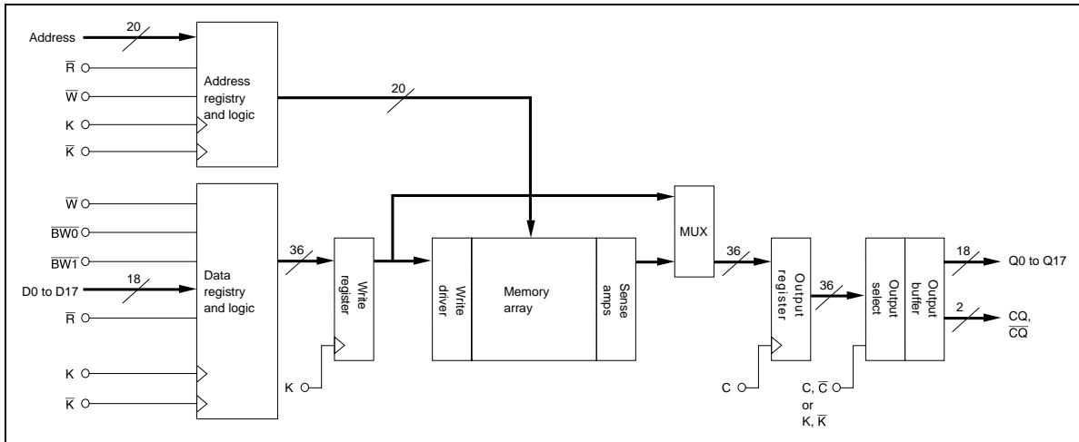
Block Diagram (HM66AQB18202)
