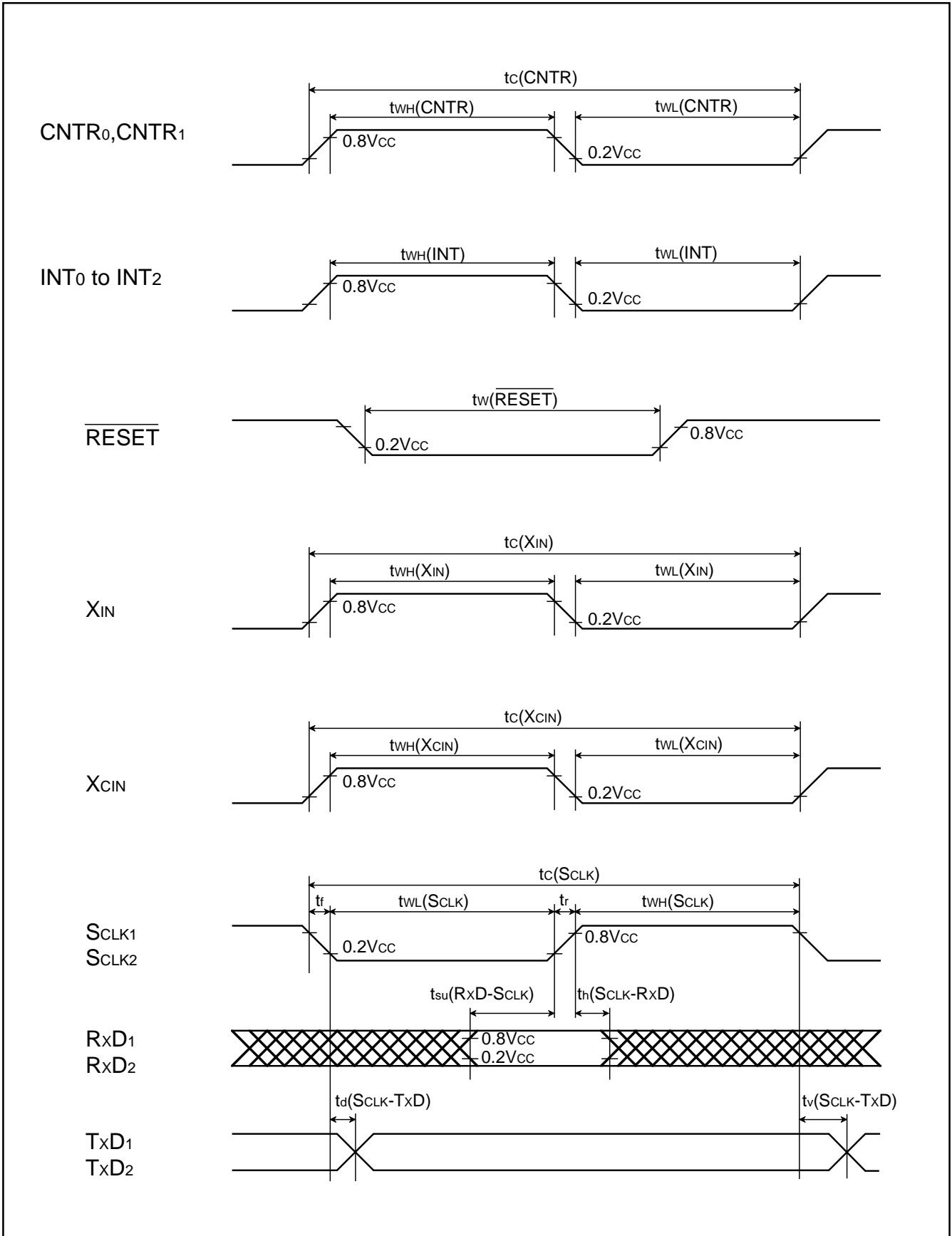
Fig. 84 Timing chart
