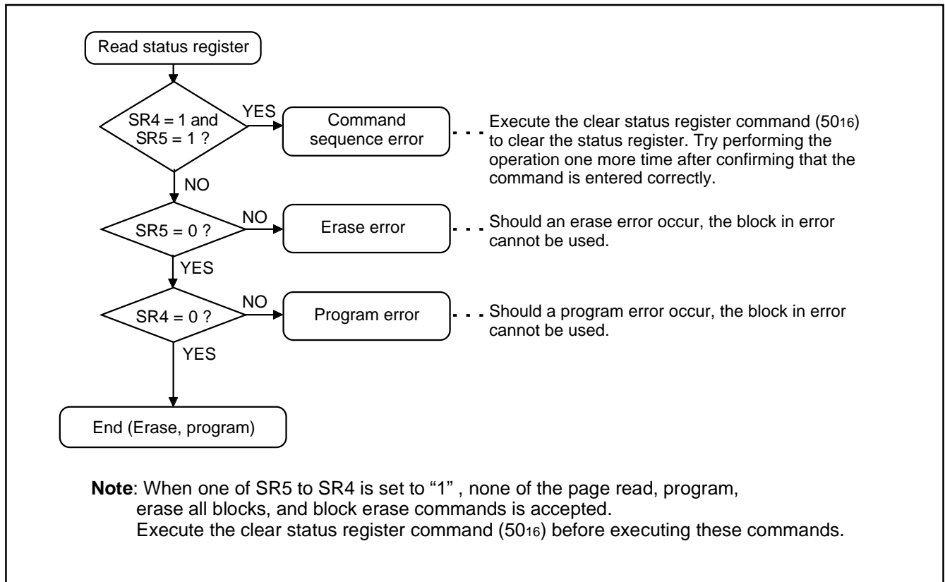
Fig. 81 Full status check flowchart and remedial procedure for errors
