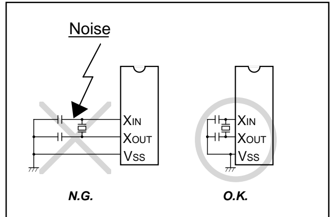
Fig. 57 Wiring for clock I/O pins
