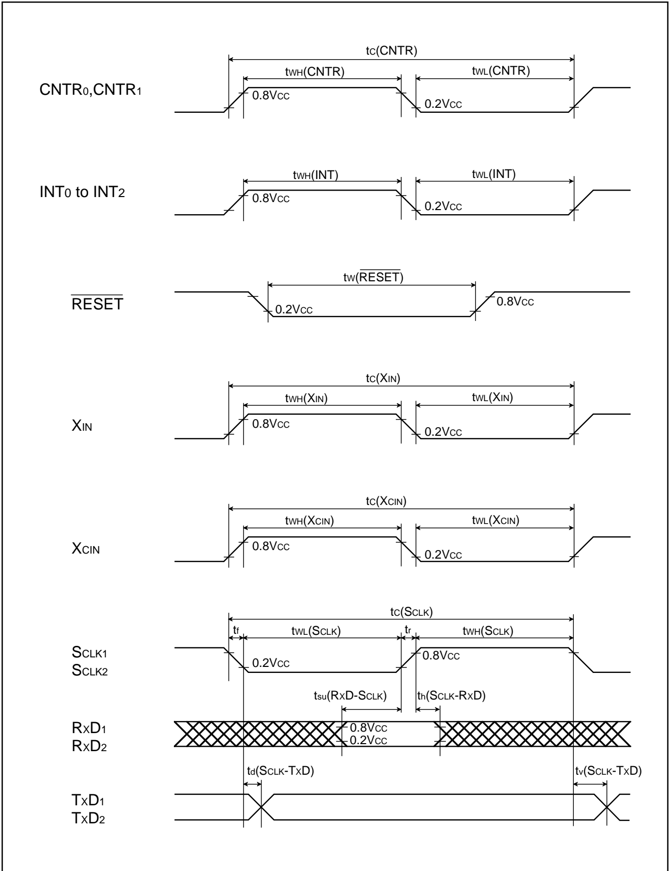
Fig. 86 Timing chart
