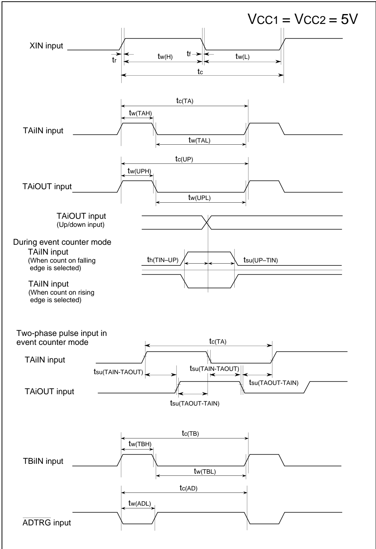
Figure 5.2 Timing Diagram (1)
