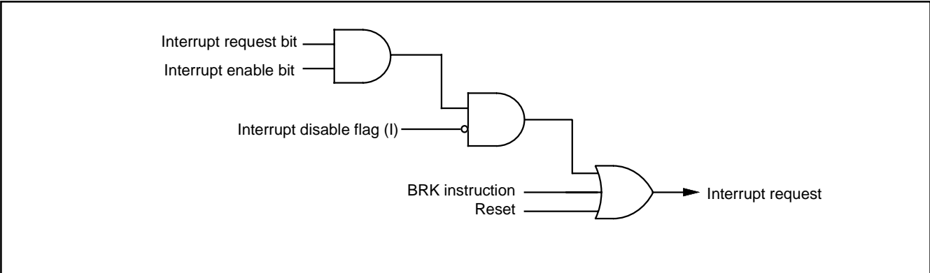
Fig. 13 Interrupt control
