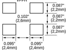
Recommended Solder Pad Layout VFFH
