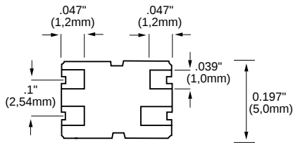
Recommended Solder Pad Layout VFFE
