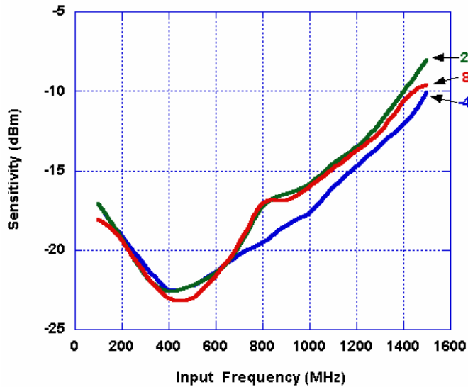
Figure 6. Input Sensitivity
