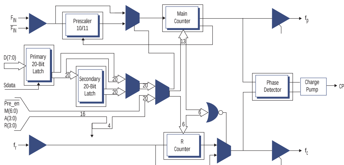
FIGURE 1. PE9701 BLOCK DIAGRAM
