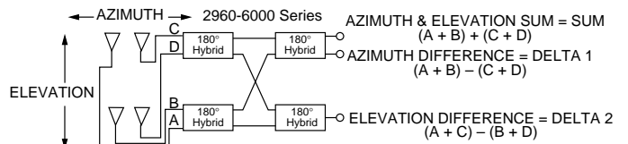
Monopulse Comparator Network
