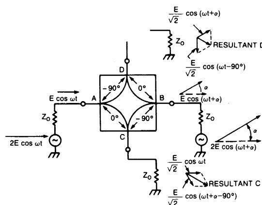
Figure 8. 90° Hybrid
