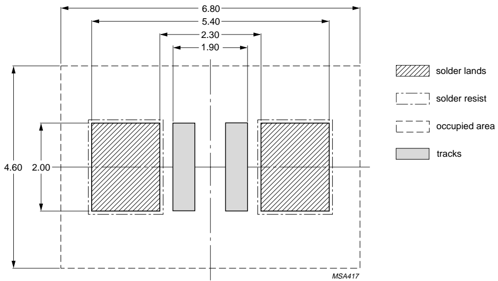
Fig.20 Wave soldering footprint for SOD87.
