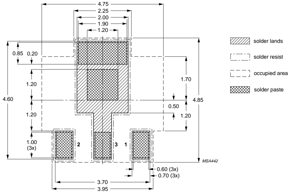
Fig.31 Reflow soldering footprint for SOT89.
