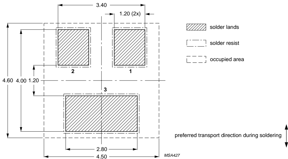
Fig.30 Wave soldering footprint for SOT23.
