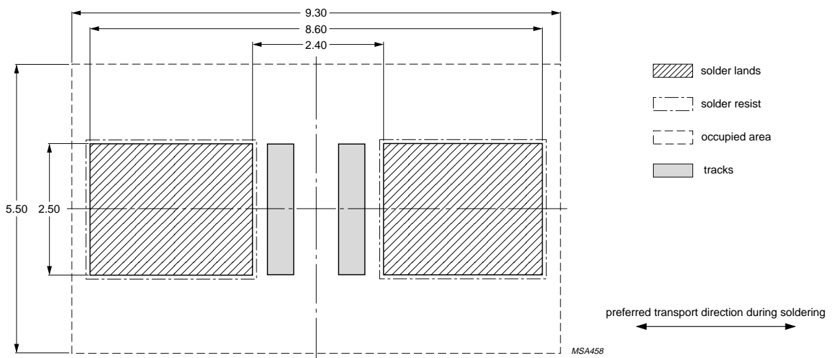
Fig.24 Wave soldering footprint for SOD106(A).
