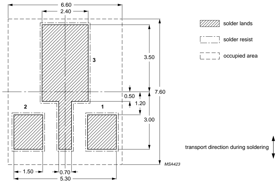
Fig.32 Wave soldering footprint for SOT89.
