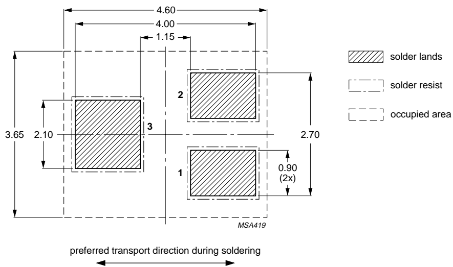
Fig.38 Wave soldering footprint for SOT323 and SC70-3.
